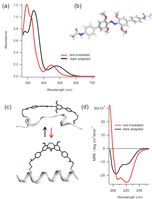
Figure 3. (a) UV-vis spectra of cross-linked with 3 . Dark-adapted (trans) spectra and red-light-irradiated (635 nm, 90 mW/cm 2 for 5 min) spectra in 5 mM NaPi buffer pH 7.0, 20 °C. (b) X-ray structure of trans 3-rf . (c) Model of FK11 cross-linked with 3 in trans and cis states. (d) CD spectra of 3 -cross-linked FK11 showing a red-light-driven increase in helix content.
