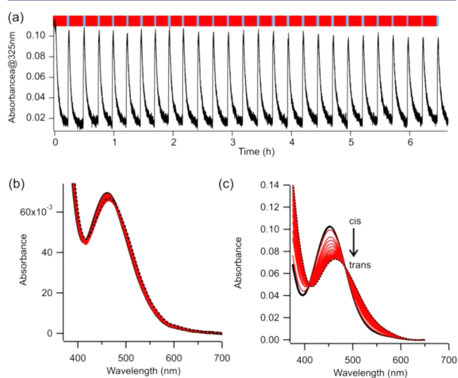
Figure 5. Stability to photobleaching and to reduction by glutathione of 4 -cross-linked FK11 (a) Multiple cycles of red-/blue-light switching in 10 mM phosphate buffer, pH 7. (b) Photoswitch 4 , in the trans state, cross-linked to FK11 was incubated in 10 mM reduced glutathione for 16 h at 25 °C. The first scan is shown as a solid black line. Intermediate scans are shown as red lines. The final scan is shown as a black dotted line. No change is evident. Normal red/blue light photoswitching (as in Figure 4) was observed after this incubation. (c) Photoswitch 4 , in the cis state, cross-linked to FK11 was incubated in 10 mM reduced glutathione for 16 h at 25 °C. Thermal cis-to-trans isomerization also occurs over this time period. Normal red-/blue-light photoswitching was observed after this incubation.
